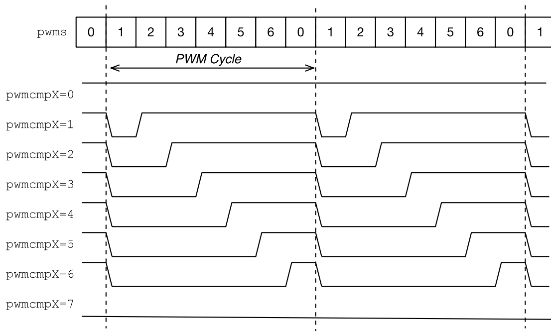
Figure 30: Basic right-aligned PWM waveforms. All possible base waveforms are shown for a 7-clock PWM cycle ( pwnmcmp0=6 ). The waveforms show the single-cycle delay caused by registering the comparator outputs in the pwnmcmpXip bits. The signals can be inverted at the GPIOs to generate left-aligned waveforms.
