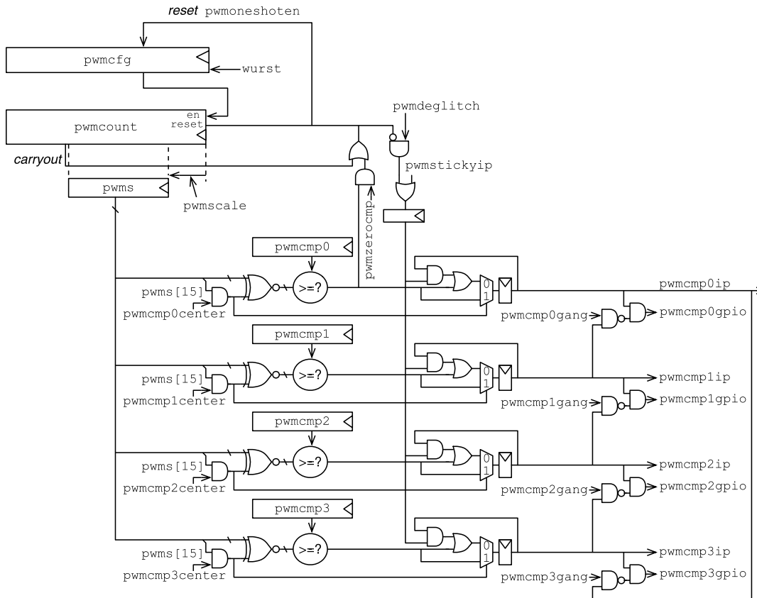
Figure 29: PWM Peripheral
